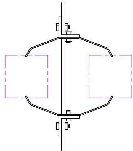
2-Point Contact Assembly
