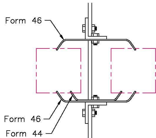
3-Point Contact Assembly
